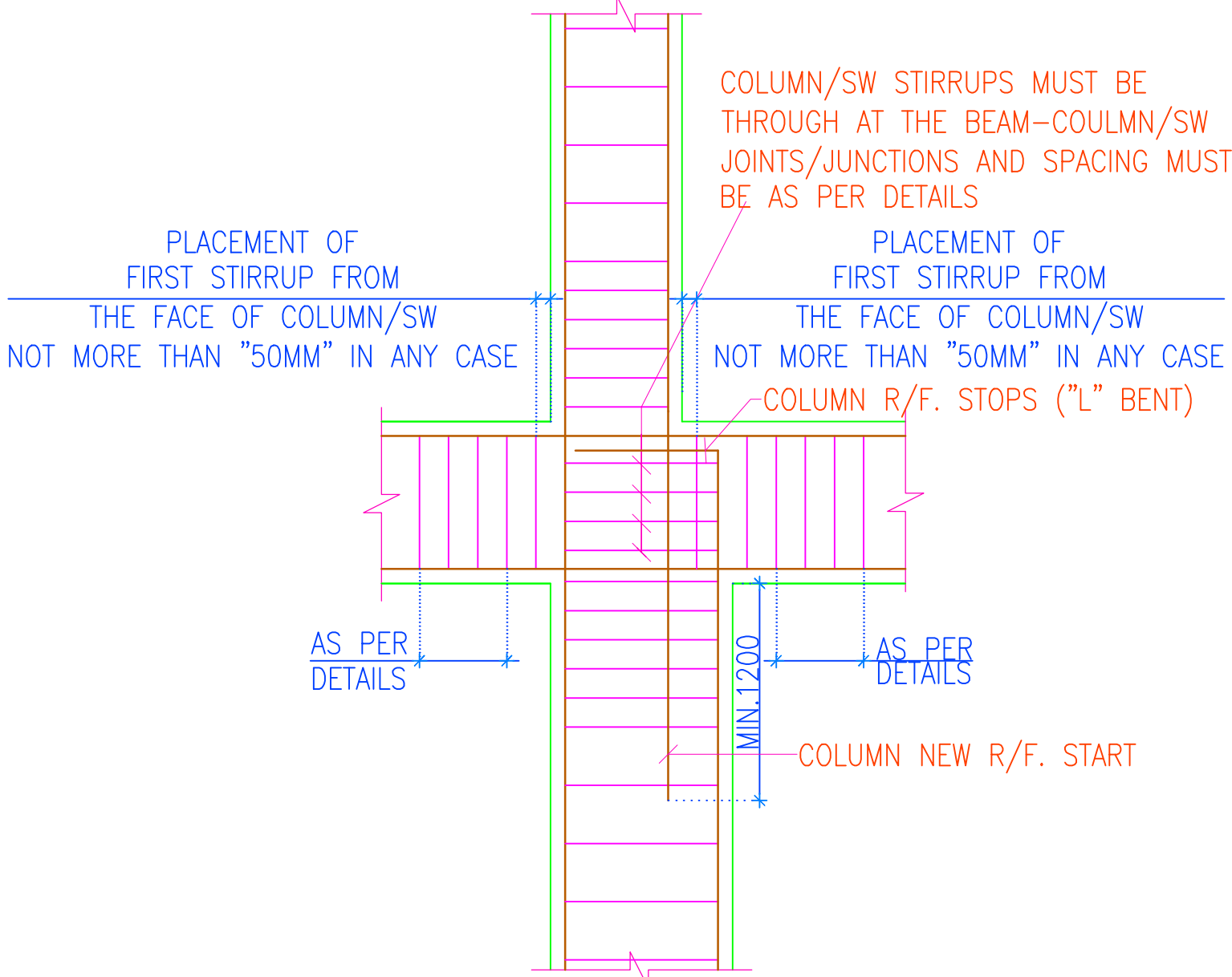
TYPICAL DETAILS FOR STIRRUPS AT REDUCTION OF COLUMNS/SHEAR WALLS (ONE SIDE)
