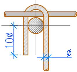
FOR 180° HOOK
