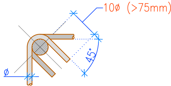
FOR 135° HOOK
