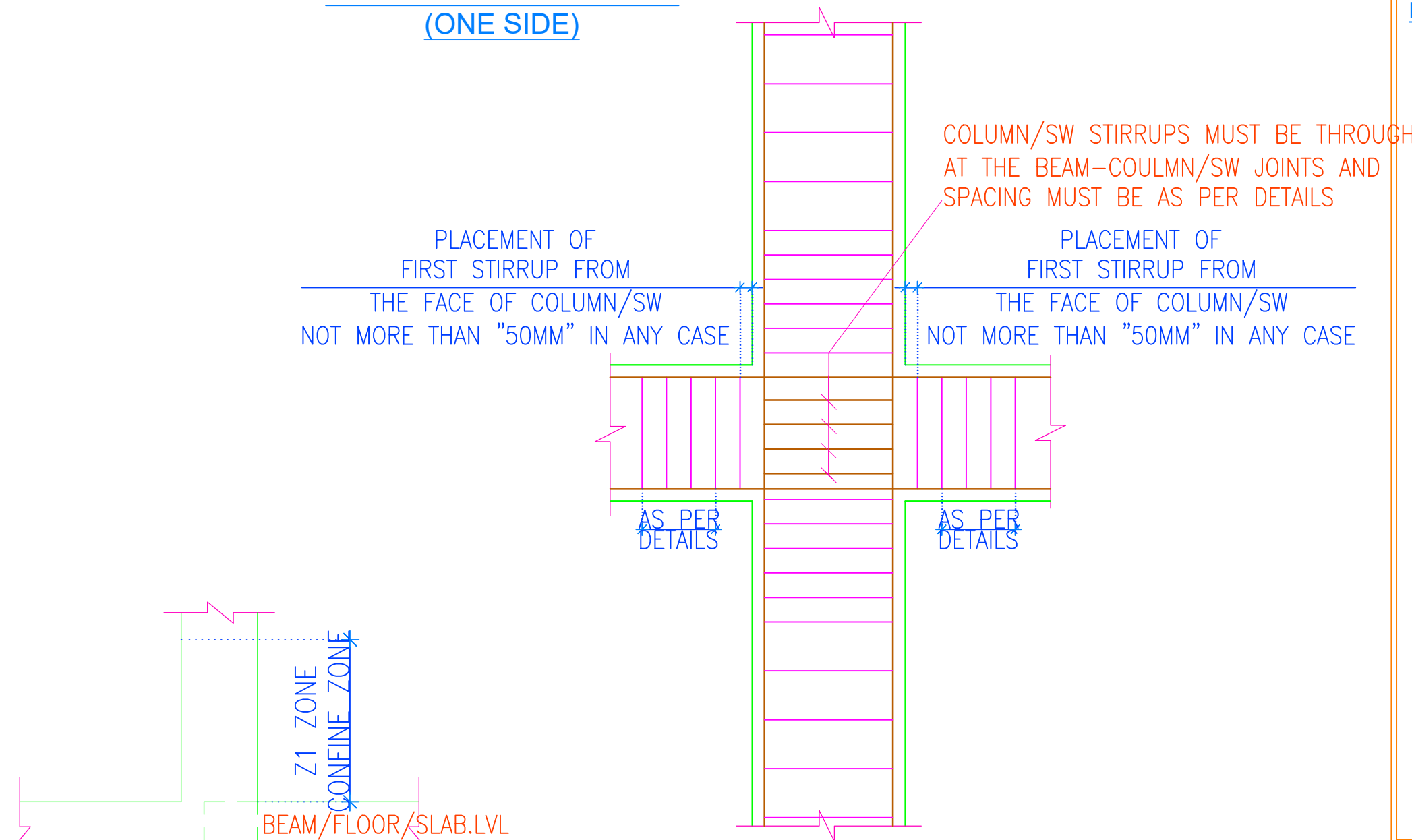
TYPICAL DETAILS FOR STIRRUPS PLACEMENTS FOR BEAMS AND COLUMNS
